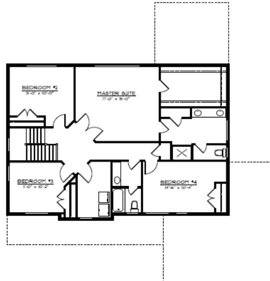
SECOND FLOOR PLAN GLENRIDGE MODEL
