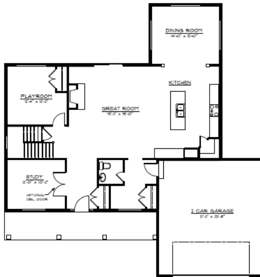
FIRST FLOOR PLAN GLENRIDGE MODEL
