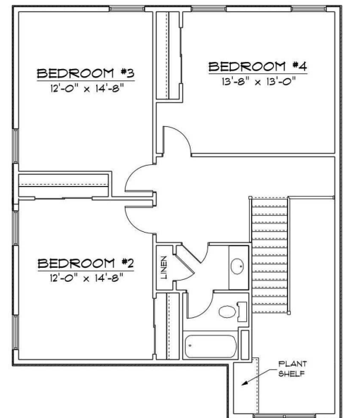
SECOND FLOOR PLAN LARGER BEDROOM OPTION
